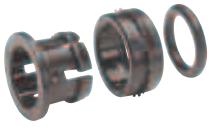
Black Acetal Collet, Black Acetal Body, Nitrile 'O' Ring.
